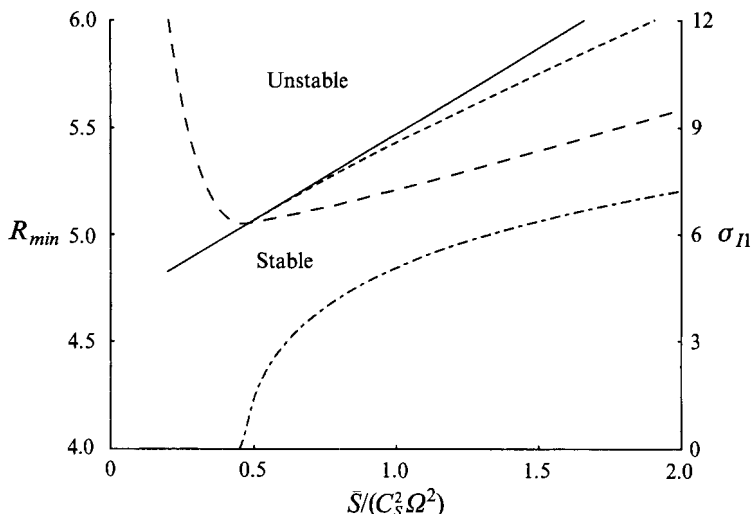
FIGURE 4. Critical Rayleigh number vs. \bar{S}/(C_S^2\Omega^2) for \delta = 0.2 and K_1 = \bar{S} = C_S . The figure indicates the loci of the minimum value of the Rayleigh number corresponding to the real mode (solid curve), the oscillatory mode (long-dashed curve) and the transition boundary (short-dashed curve) which can be associated with the sketches in figure 3. These curves correspond to the left-hand-side axis. Also indicated, and corresponding to the right-hand-side axis, is the frequency \sigma_{11} (dashed-dotted curve) along the oscillatory branch. There is a transition point near \bar{S}/(C_S^2\Omega^2) = 0.5 below which the minimum of the transition boundary and the minimum of the neutral stability curve for the oscillatory mode coincide and above which the three curves separate.
